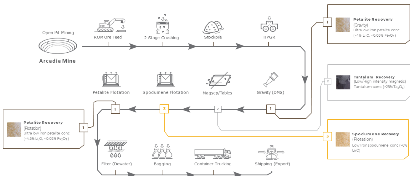
Figure 1: Proposed Metallurgical Flowsheet
